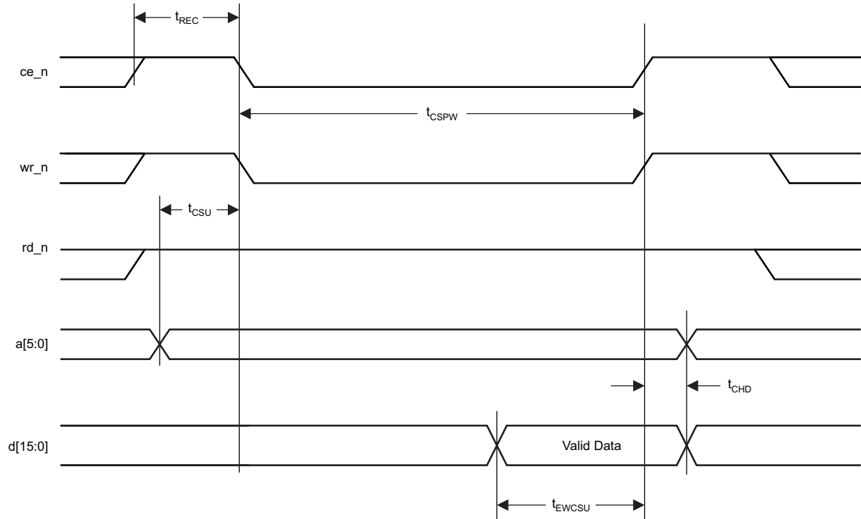
Figure 8-3. Write Operation—3-Pin Control Mode
